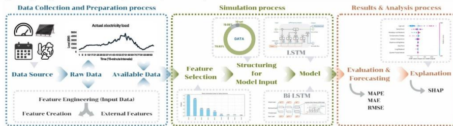
Fig.4: The Complete Forecasting Process
