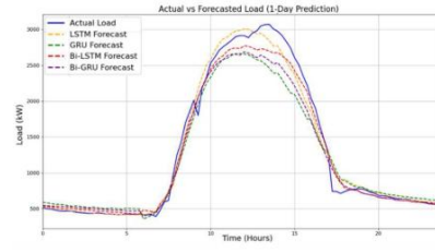
Fig. 6. One-day-ahead electrical load forecast for each model on weekdays
