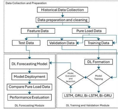
Fig. 5. The Proposed Load Forecasting Framework
