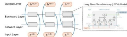
Fig.3: The Bi-LSTM Architecture
