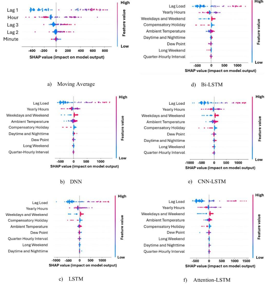
Fig.9: Shap Value of Each Model:
