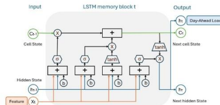
Fig.2: The LSTM Architecture
