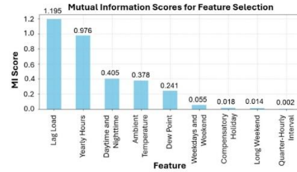
Fig.5: Mutual Information Scores
