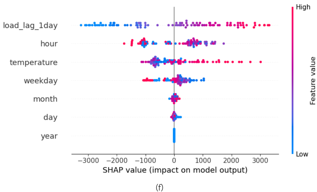
Figure D.2 SHAP Value of Each Model of ISO-NE Data: a) Moving average, b) DNN, c) LSTM, d) Bi-LSTM, e) CNN-LSTM, and f) Attention-LSTM (continued)
