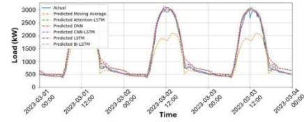
Fig.8: The Best-Performing Forecasting Results in the Test Set during the Exam Period
