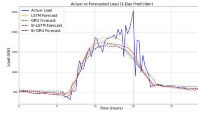
Fig. 7. One-day-ahead electricity load forecast for each model on weekends
