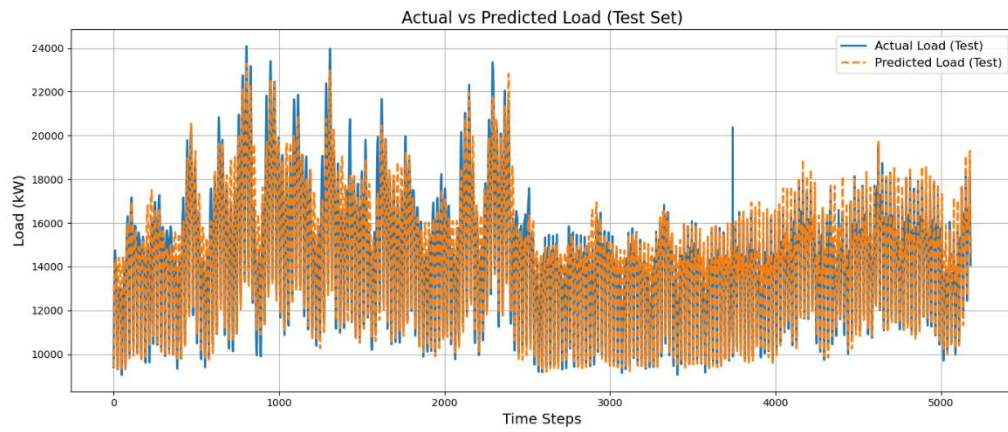
Figure C.3 Performance evaluation results for test data set of ISO-NE Data: a) Moving average, b) DNN, c) LSTM, d) Bi-LSTM, e) CNN-LSTM, f) Attention-LSTM and g) Top 3 Features
