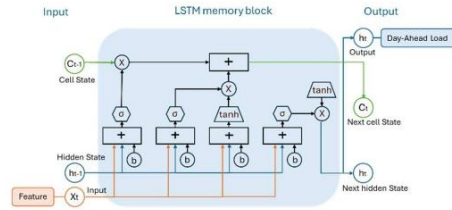
Fig. 1. LSTM architecture.
