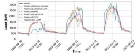
Fig.7: The Lowest-Performing Forecast Results in the Rainy Season Test Set
