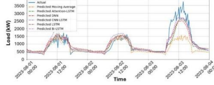
Fig.6: The Lowest-Performing Forecast Results in the Initial Semester Test Set
