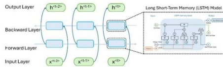
Fig. 2. Bi-LSTM architecture.
