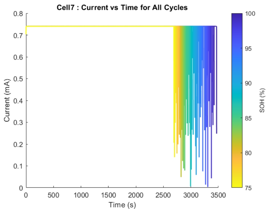
Figure A.20 Current profiles Cell 7 of Oxford are used to charge all the cycles.
