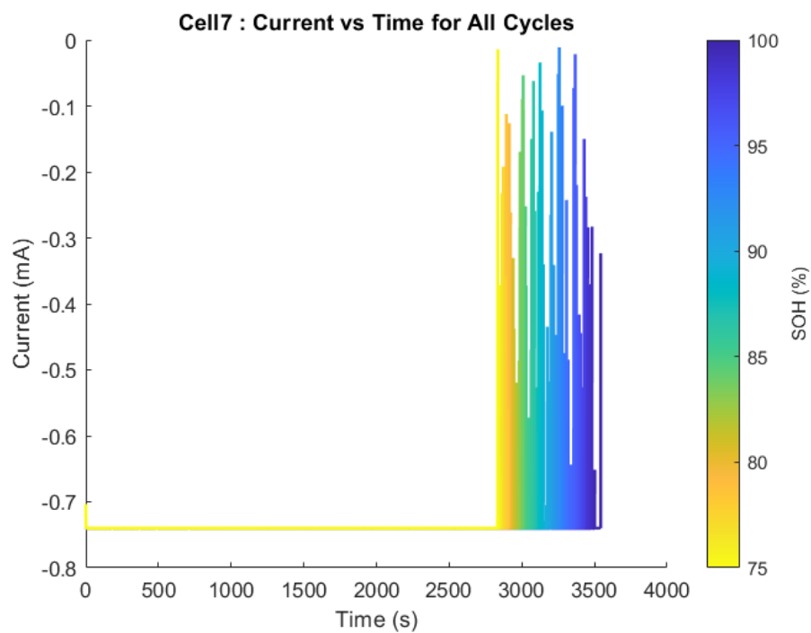
Figure A.27 Current profiles Cell 7 of Oxford are used to charge all the cycles.
