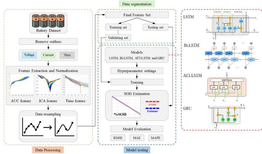
Fig.1: Overall Framework of the Proposed Battery SOH Estimation
