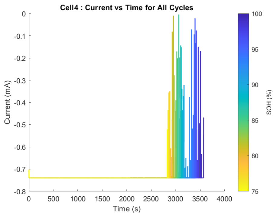
Figure A.24 Current profiles Cell 4 of Oxford are used to discharge all the cycles.
