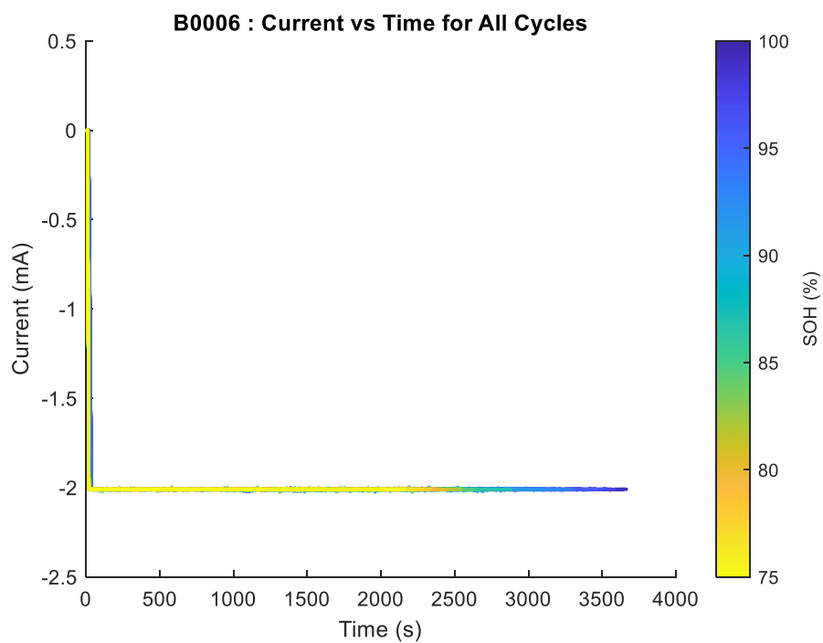
Figure B.10 Current profiles B0006 of NASA are used to discharge all the cycles.
