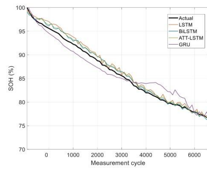
Fig.12: SOH Estimation Results at the Worst Interval
