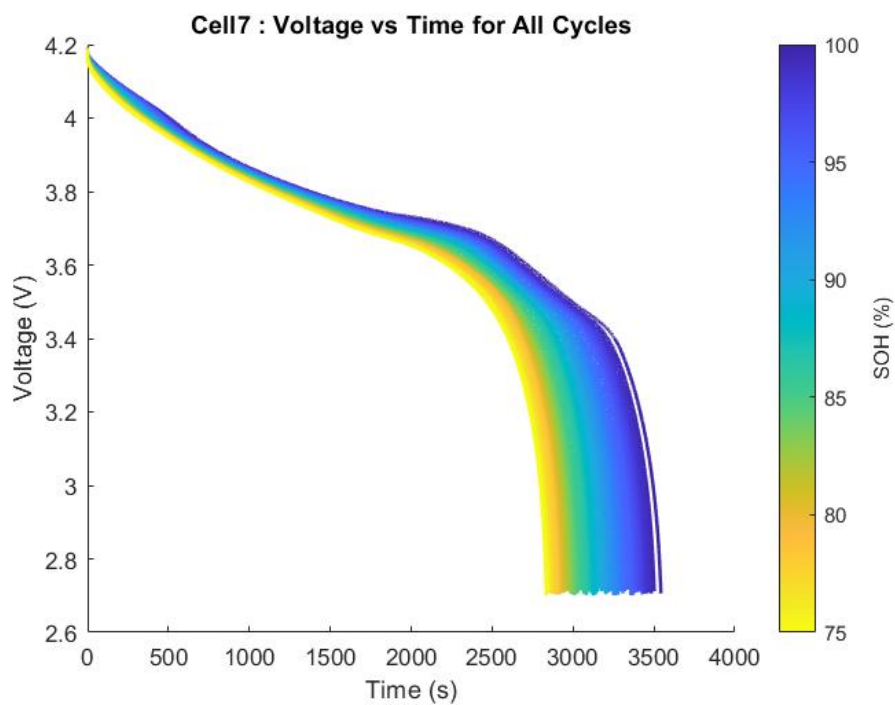
Figure A.13 Voltage profiles Cell 7 of Oxford are used to discharge all the cycles.
