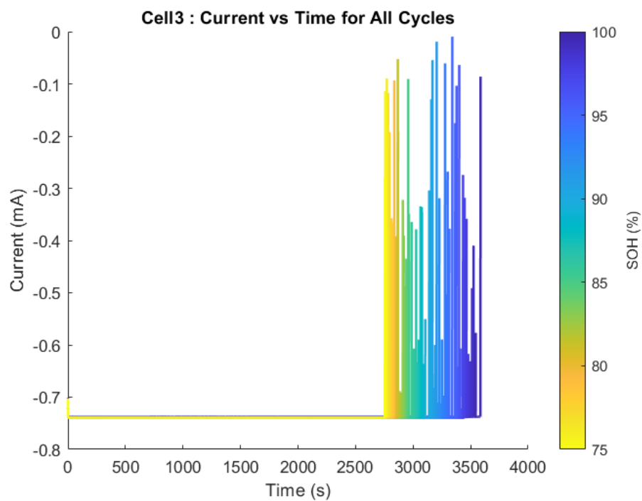
Figure A.23 Current profiles Cell 3 of Oxford are used to charge all the cycles.
