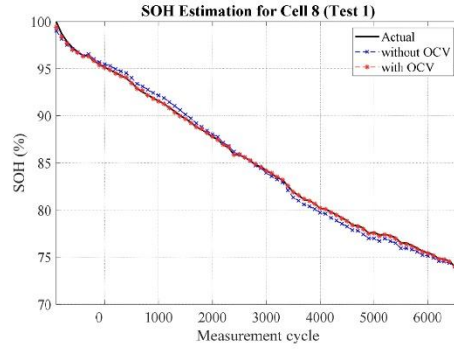
Fig. 6. SOH estimation of Cell 8 (Test 1).
