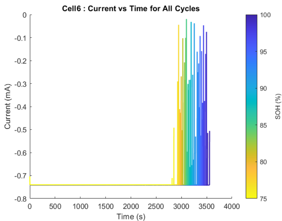
Figure A.26 Current profiles Cell 6 of Oxford are used to discharge all the cycles.
