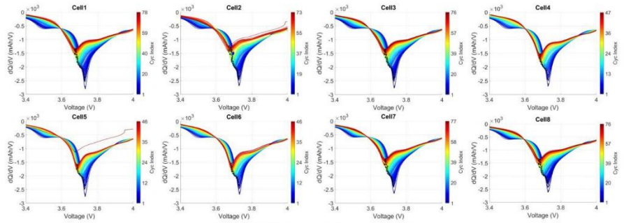
Fig.5: ICA Curve all the cycles 8 cells
