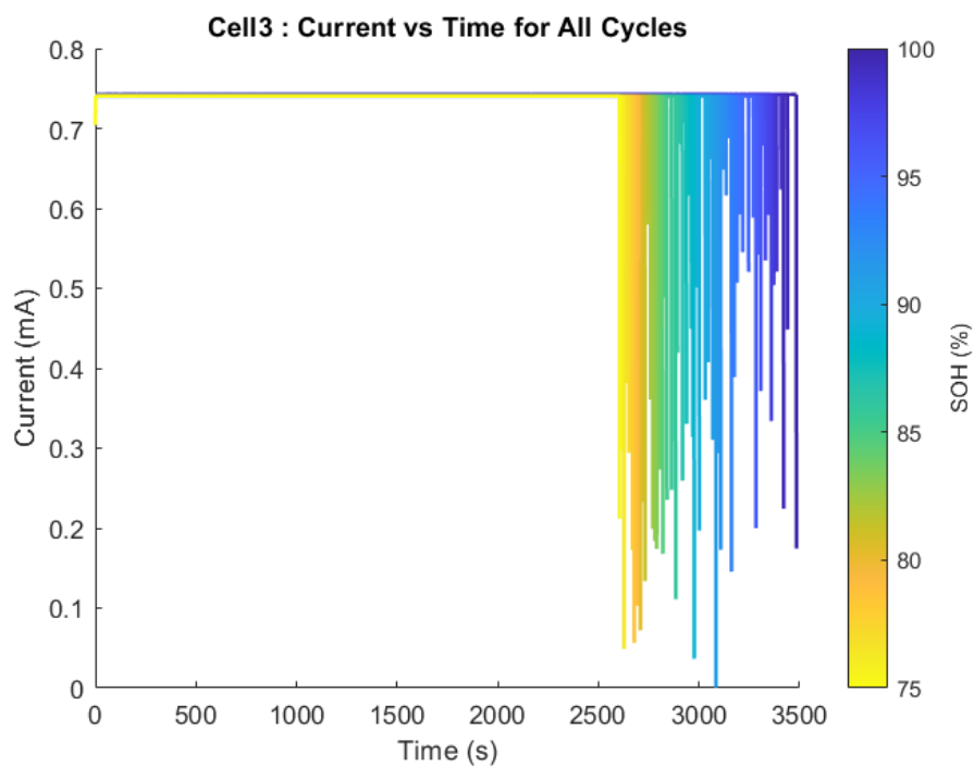
Figure A.16 Current profiles Cell 3 of Oxford are used to charge all the cycles.
