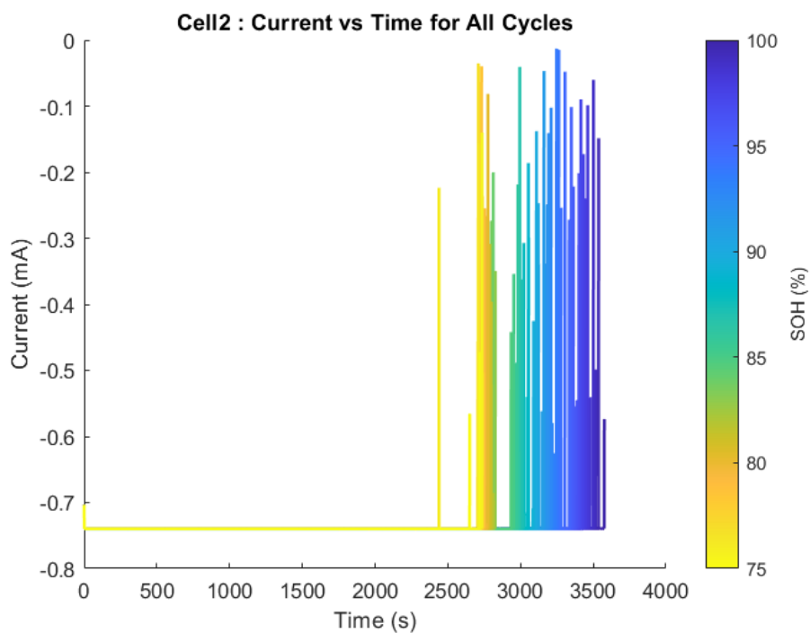
Figure A.22 Current profiles Cell 2 of Oxford are used to discharge all the cycles.
