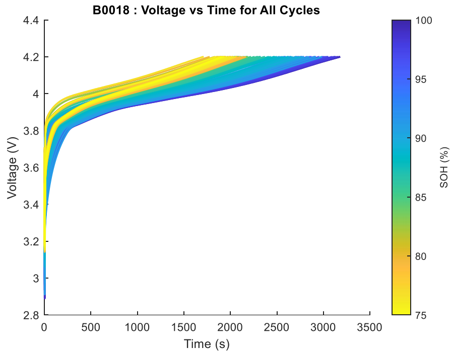
Figure B.3 Voltage profiles B0018 of NASA are used to charge all the cycles.
