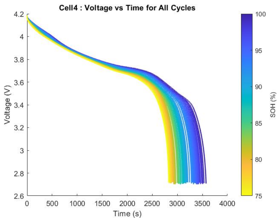
Figure A.10 Voltage profiles Cell 4 of Oxford are used to discharge all the cycles.
