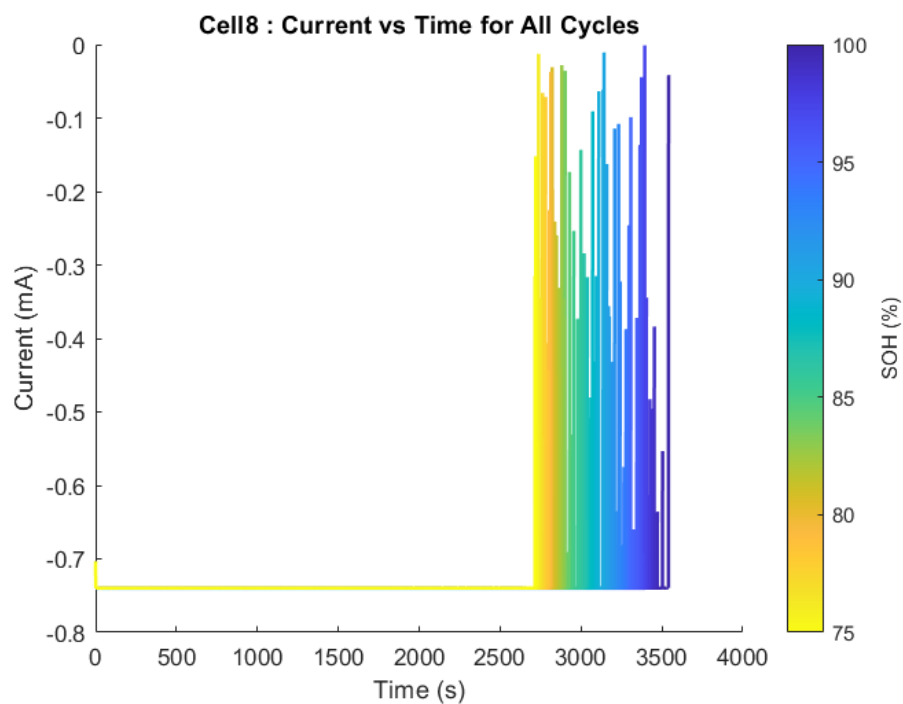
Figure A.28 Current profiles Cell 8 of Oxford are used to discharge all the cycles.
