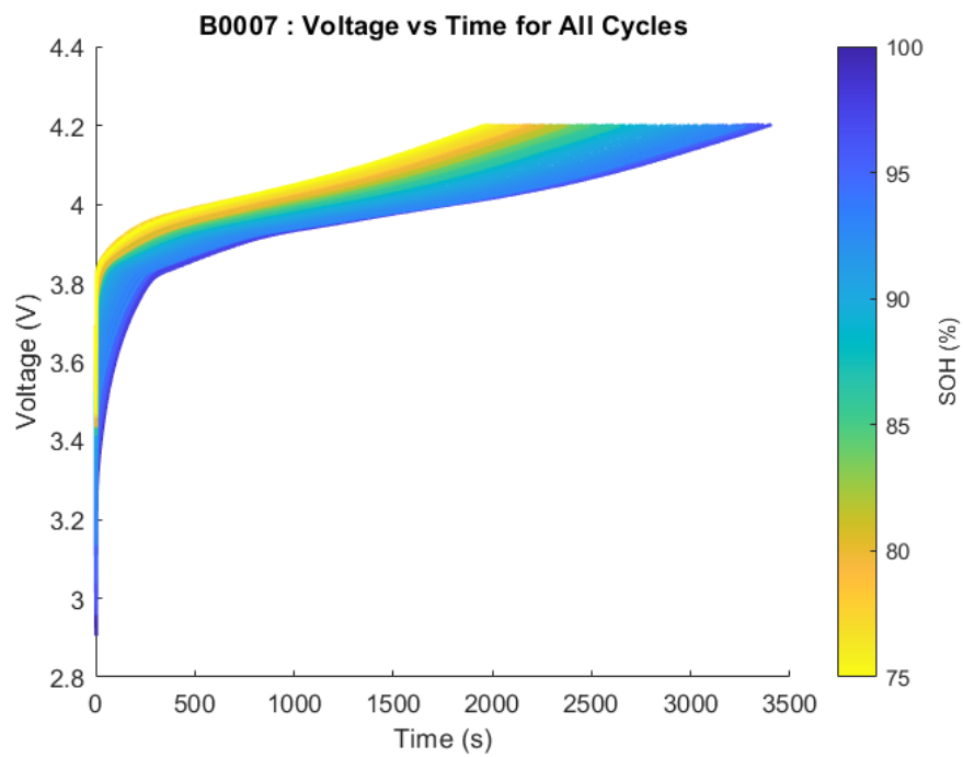
Figure B.2 Voltage profiles B0007 of NASA are used to charge all the cycles.
