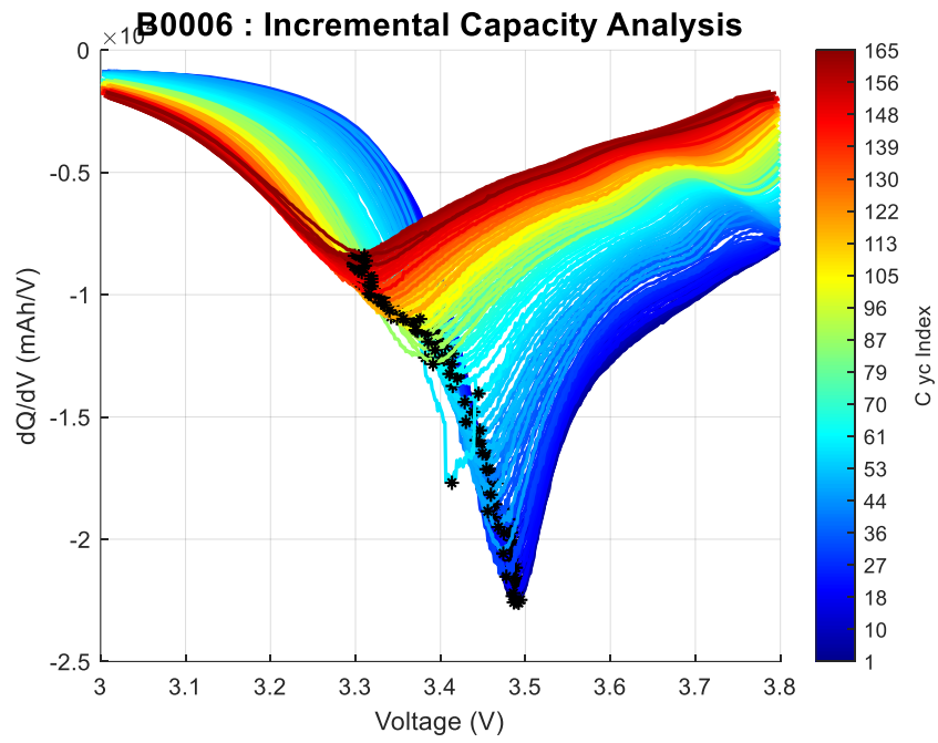
Figure D.1 ICA curves for NASA B0006.
