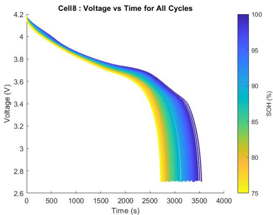
Figure A.14 Voltage profiles Cell 8 of Oxford are used to discharge all the cycles.
