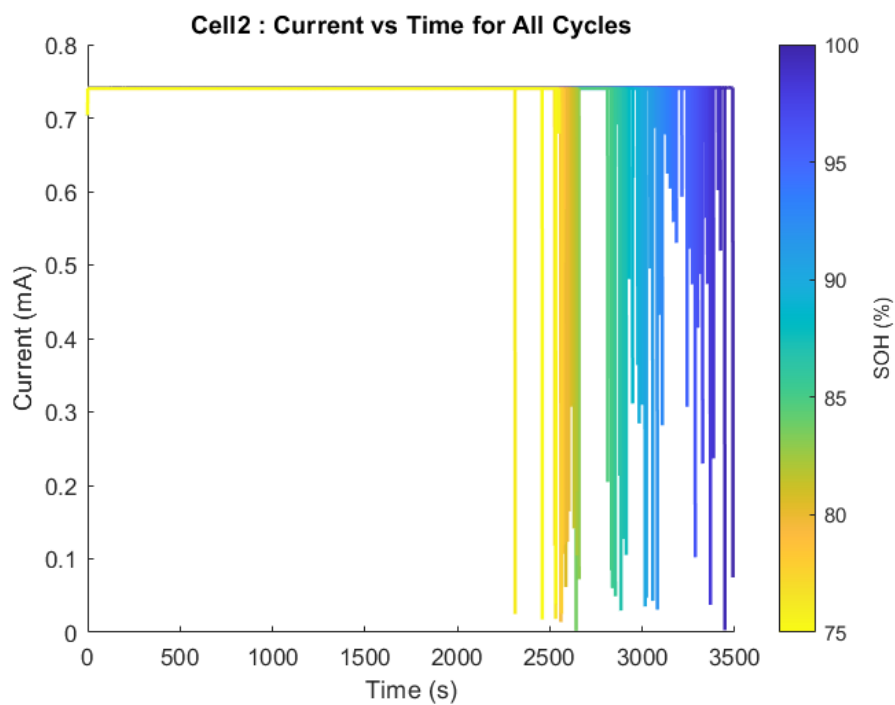
Figure A.15 Current profiles Cell 2 of Oxford are used to charge all the cycles.
