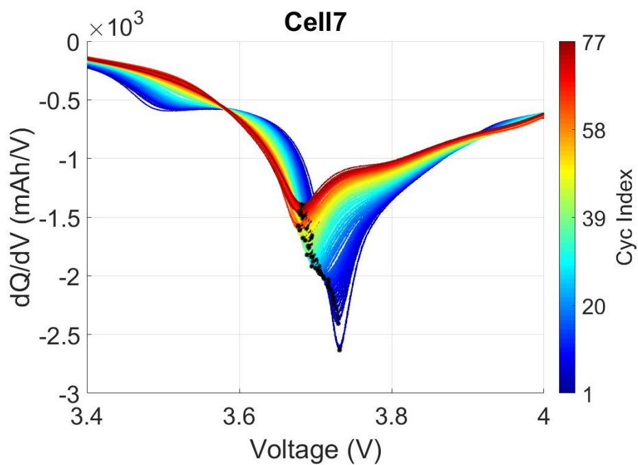
Figure C.6 ICA curves for Oxford Cell 7.
