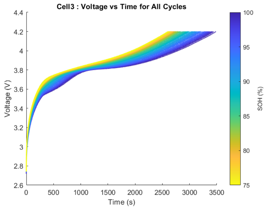
Figure A.2 Voltage profiles Cell 3 of Oxford are used to charge all the cycles.
