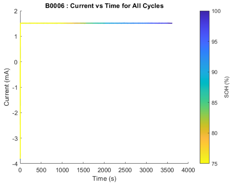
Figure B.7 Current profiles B0006 of NASA are used to charge all the cycles.
