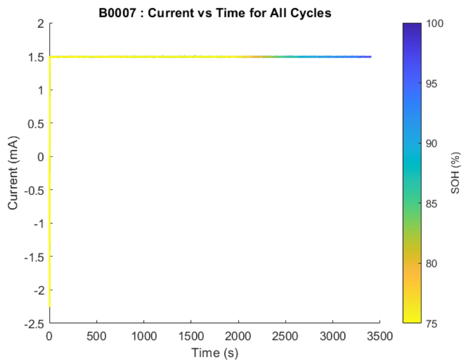
Figure B.8 Current profiles B0007 of NASA are used to charge all the cycles.
