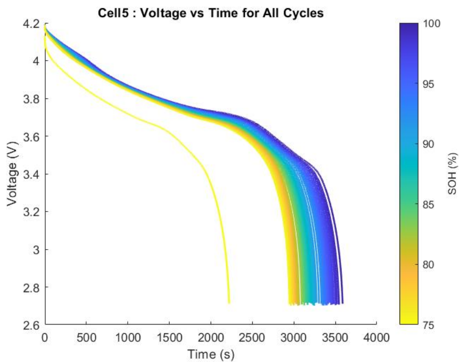
Figure A.11 Voltage profiles Cell 5 of Oxford are used to discharge all the cycles.
