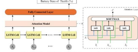
Fig.9: The ATT-LSTM Network Architecture
