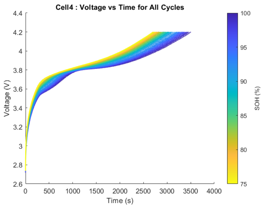
Figure A.3 Voltage profiles Cell 4 of Oxford are used to charge all the cycles.
