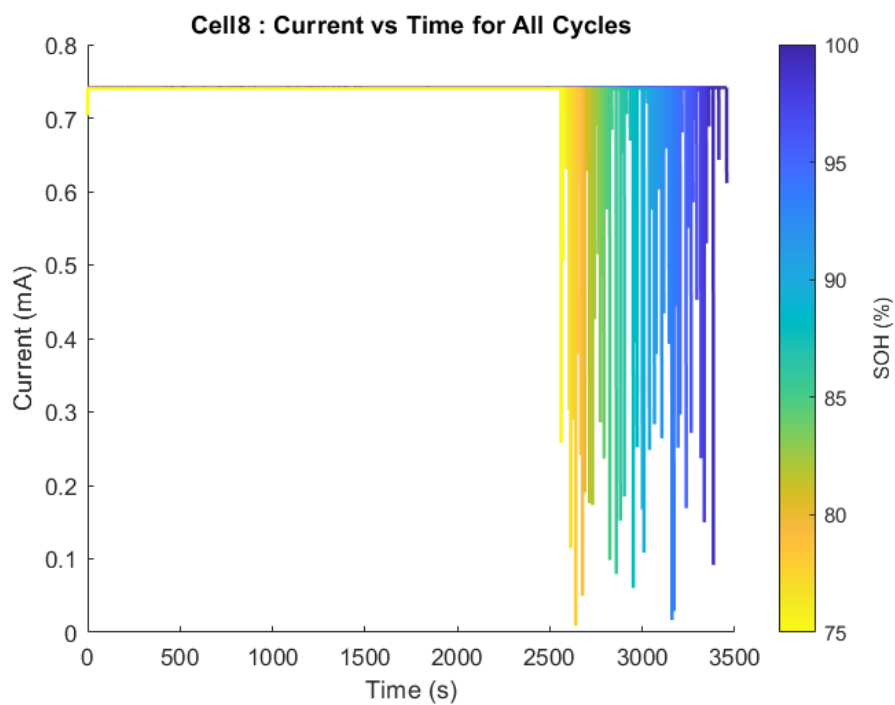
Figure A.21 Current profiles Cell 8 of Oxford are used to charge all the cycles.
