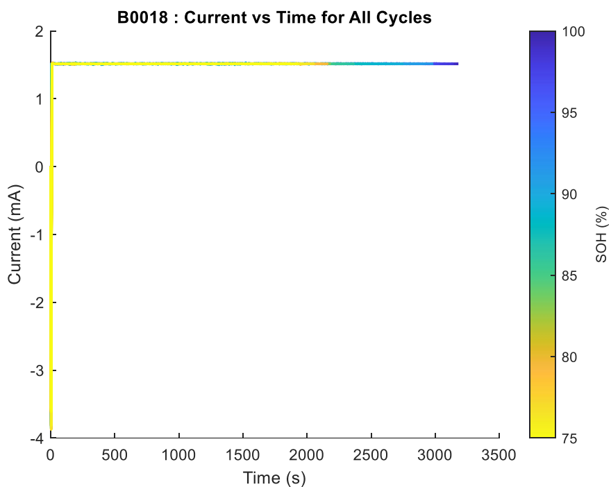
Figure B.9 Current profiles B0018 of NASA are used to charge all the cycles.
