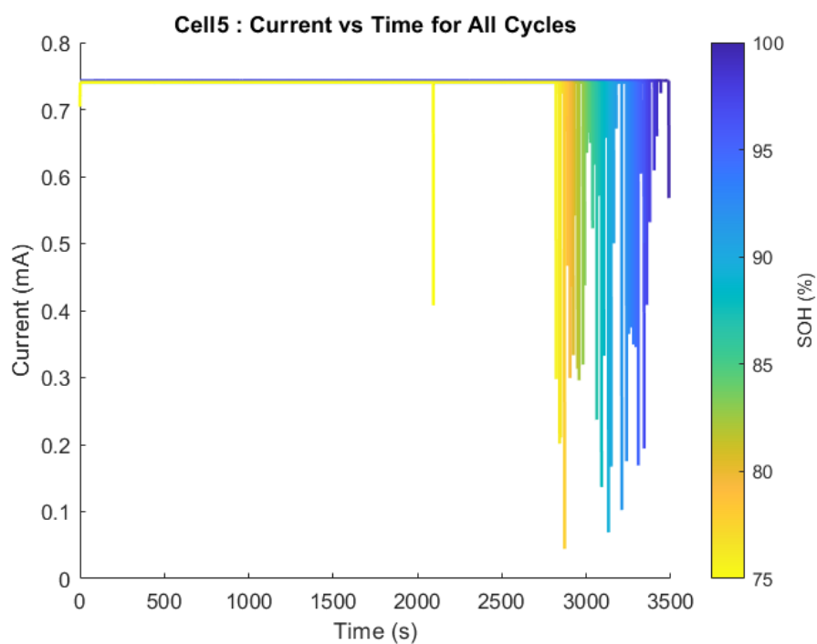
Figure A.18 Current profiles Cell 5 of Oxford are used to charge all the cycles.
