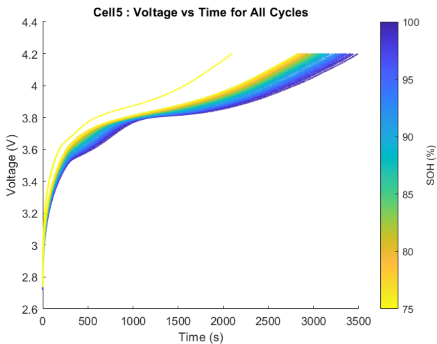
Figure A.4 Voltage profiles Cell 5 of Oxford are used to charge all the cycles.
