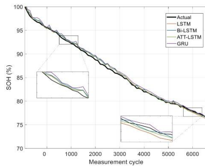
Fig.11: SOH Estimation Results at the Best Interval
