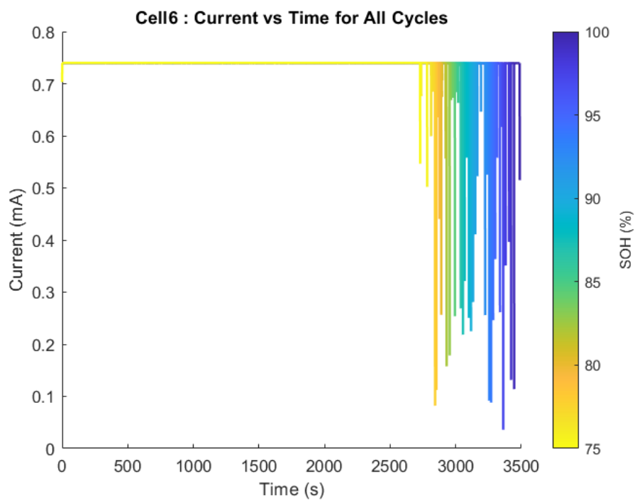
Figure A.19 Current profiles Cell 6 of Oxford are used to charge all the cycles.
