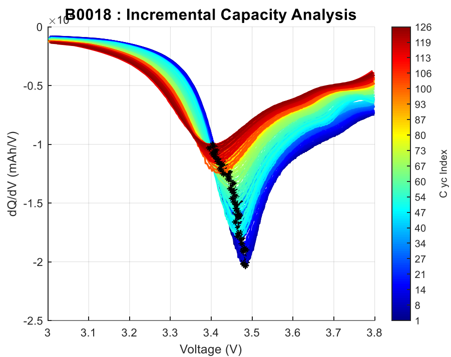
Figure D.5 ICA curves for NASA B0018.
