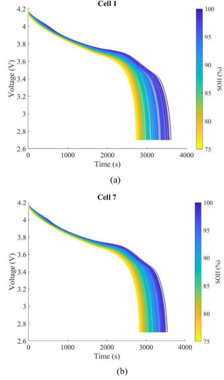
Fig. 1. (a) Voltage profiles of Cell 1 are used to discharge all the cycles. (b) Voltage profiles of Cell 7 are used to discharge all the cycles.
