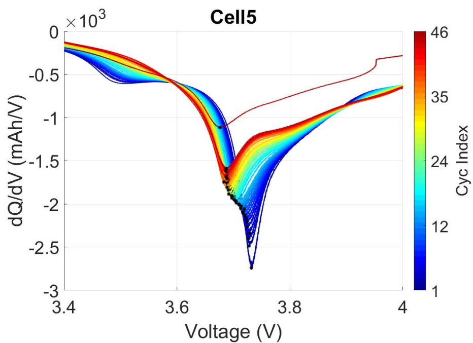
Figure C.4 ICA curves for Oxford Cell 5.
