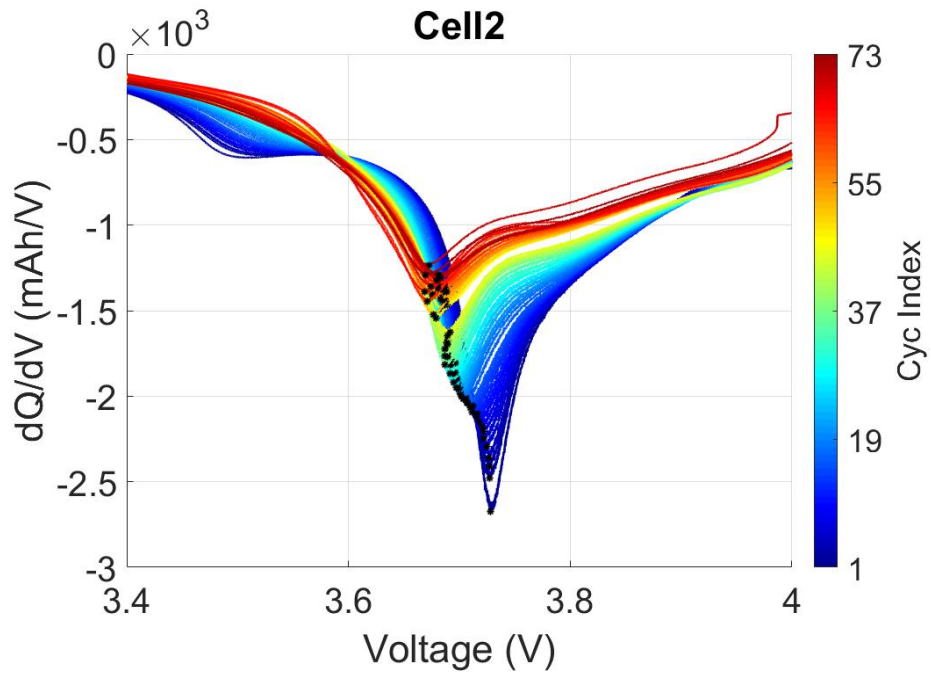
Figure C.1 ICA curves for Oxford Cell 2.
