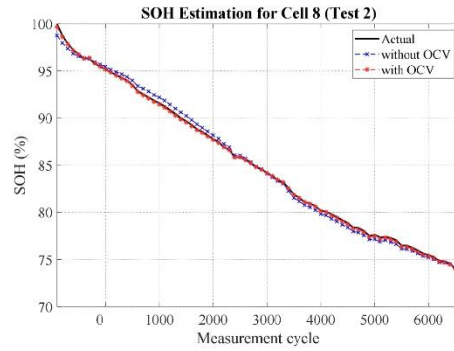
Fig. 7. SOH estimation of Cell 8 (Test 2).
