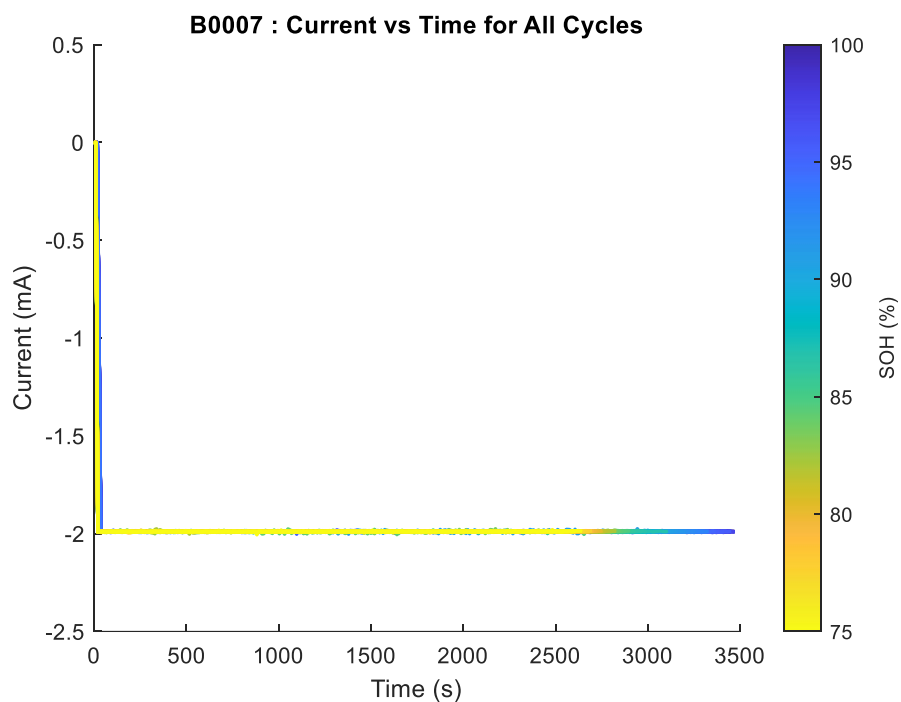
Figure B.11 Current profiles B007 of NASA are used to discharge all the cycles.
