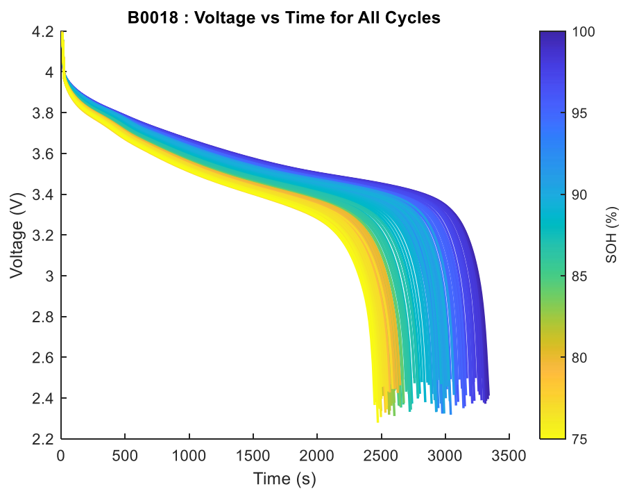
Figure B.6 Voltage profiles B0018 of NASA are used to discharge all the cycles.
