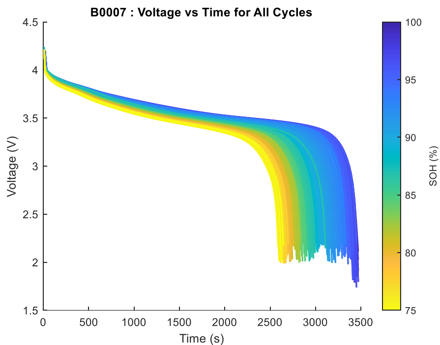
Figure B.5 Voltage profiles B0007 of NASA are used to discharge all the cycles.
