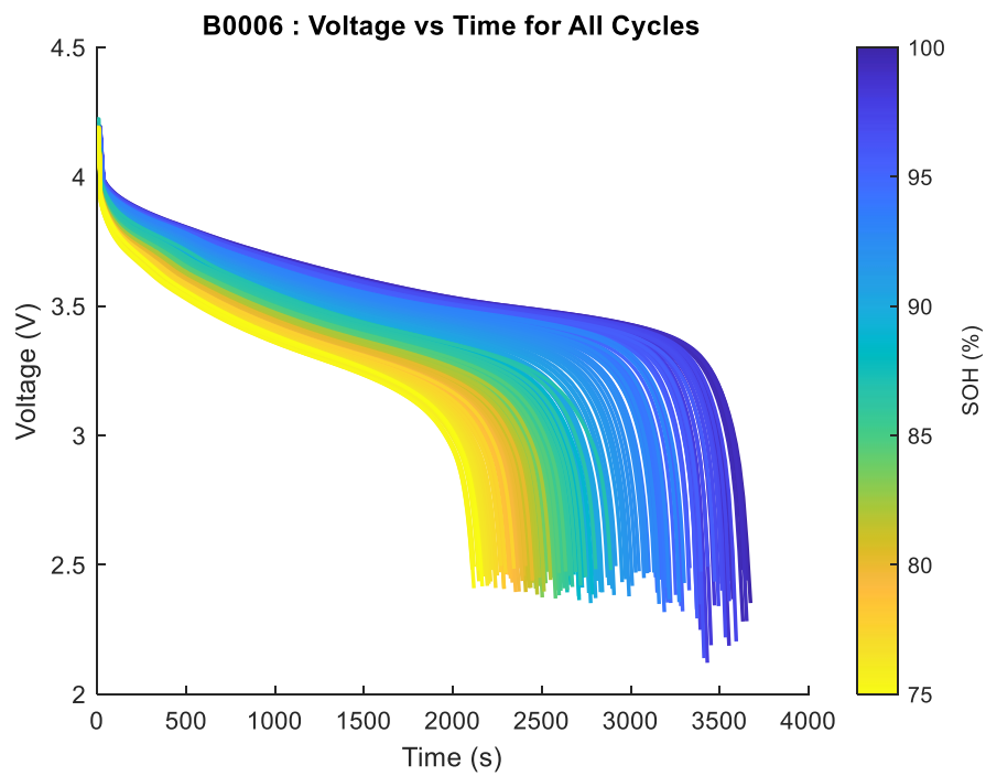
Figure B.4 Voltage profiles B0006 of NASA are used to discharge all the cycles.
