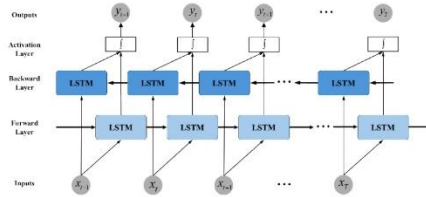
Fig.8: The Bi-LSTM Network Architecture
