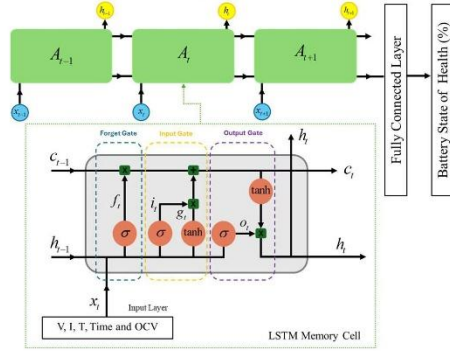
Fig. 5. An example of the LSTM cell for the SOH estimation.
