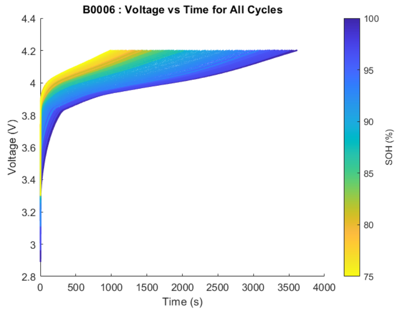
Figure B.1 Voltage profiles B0006 of NASA are used to charge all the cycles.
