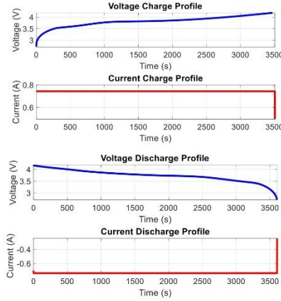
Fig. 2: Voltage and Current Profiles During Charging and Discharging cycles at a 1C rate.
