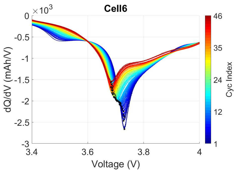
Figure C.5 ICA curves for Oxford Cell 6.
