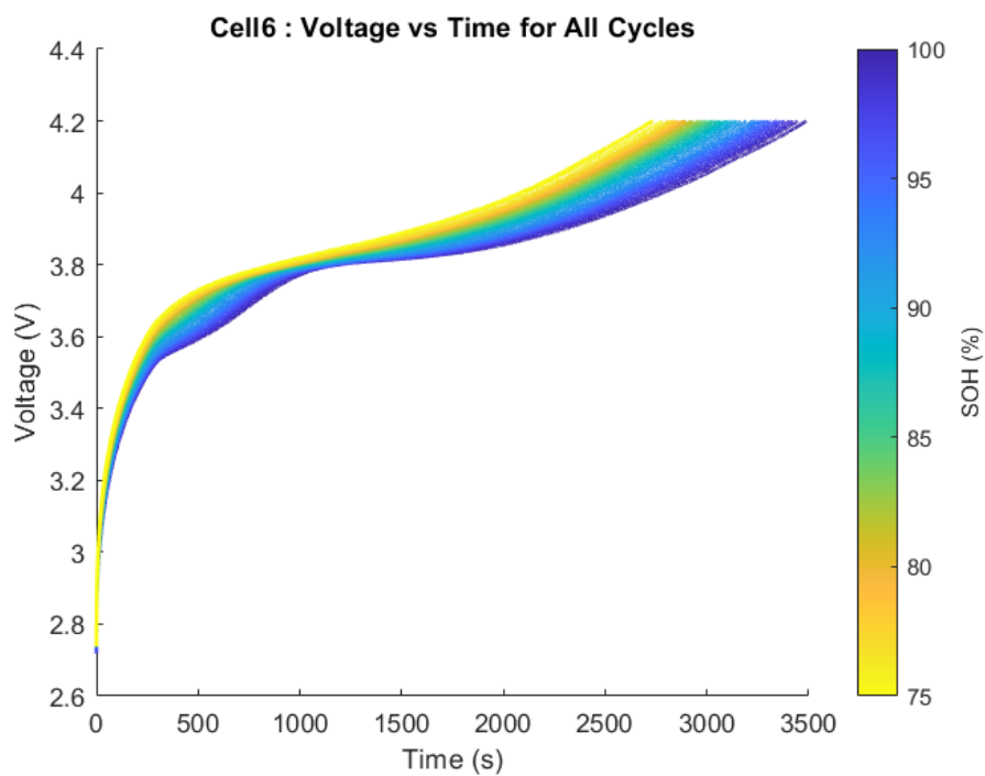
Figure A.5 Voltage profiles Cell 6 of Oxford are used to charge all the cycles.
