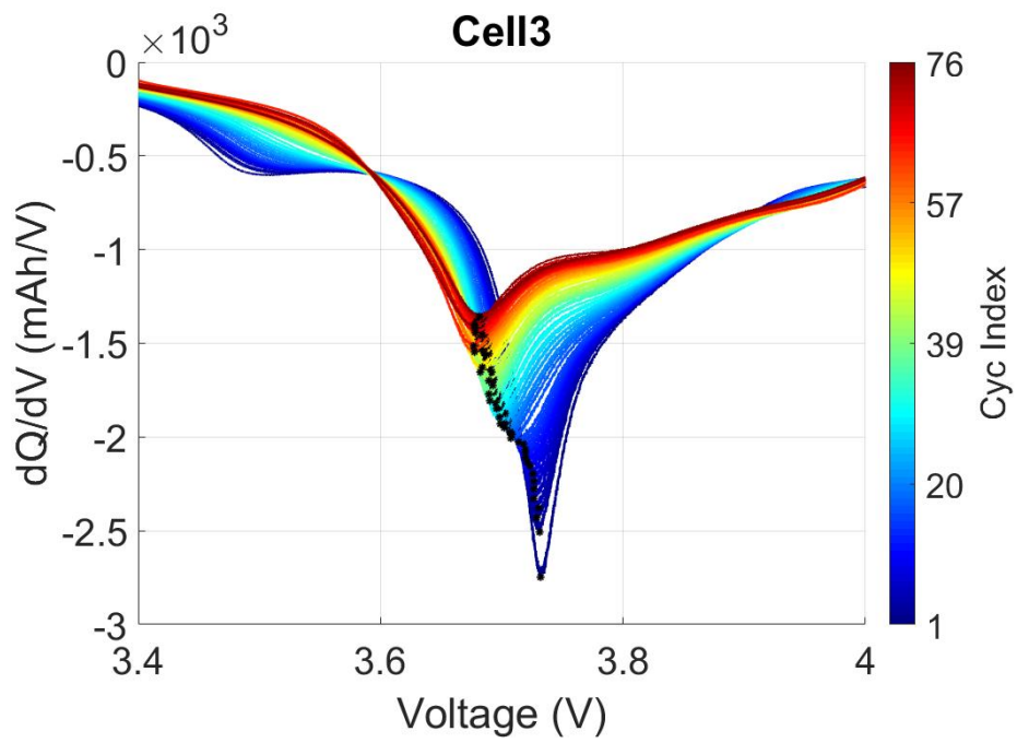
Figure C.2 ICA curves for Oxford Cell 3.
