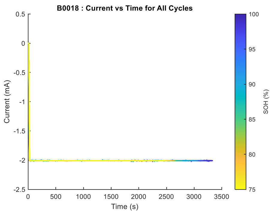
Figure B.12 Current profiles B0018 of NASA are used to discharge all the cycles.
