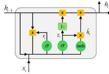
Fig.10: The GRU Network Architecture
