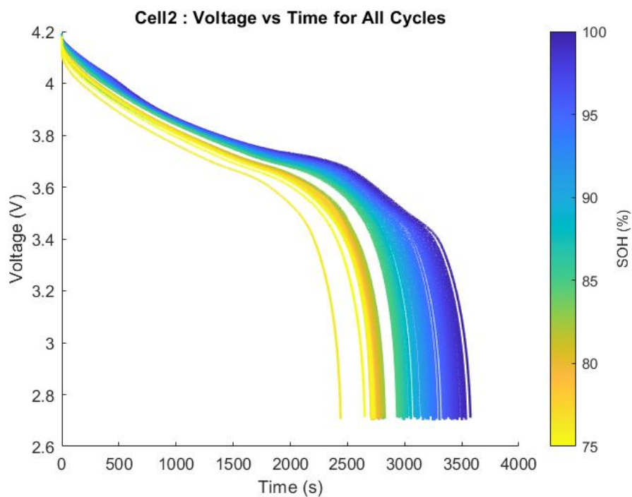
Figure A.8 Voltage profiles Cell 2 of Oxford are used to discharge all the cycles.
