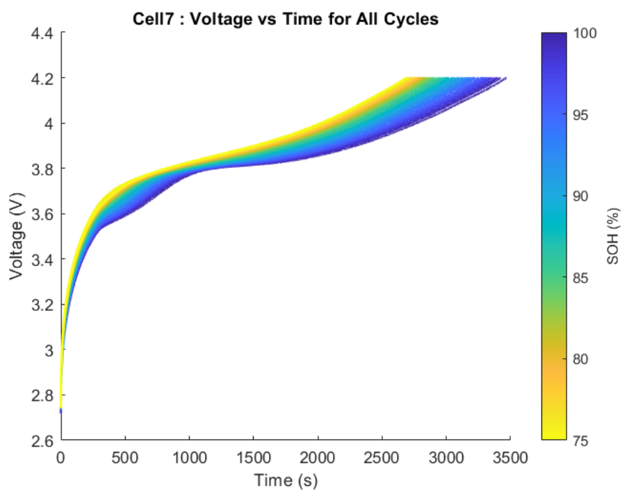
Figure A.6 Voltage profiles Cell 7 of Oxford are used to charge all the cycles.
