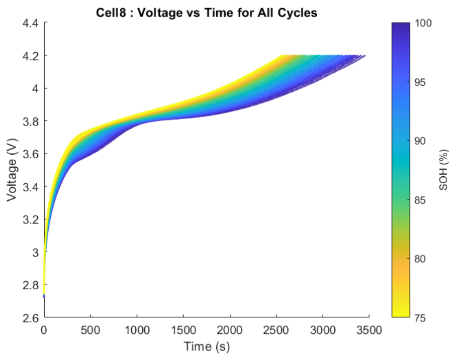
Figure A.7 Voltage profiles Cell 8 of Oxford are used to charge all the cycles.
