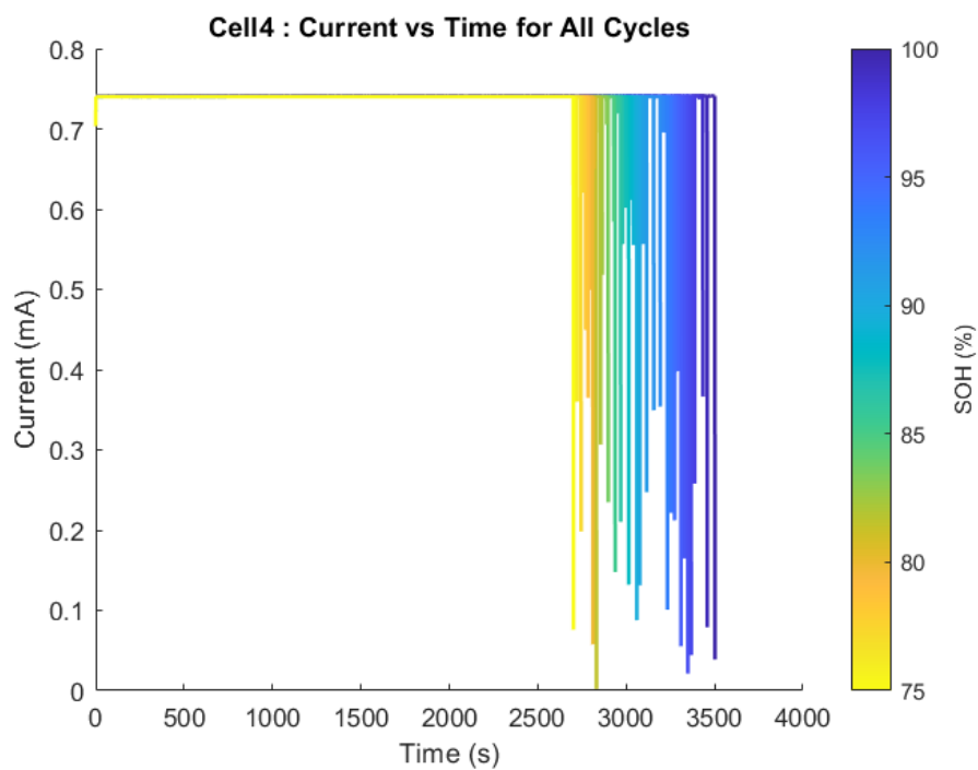
Figure A.17 Current profiles Cell 4 of Oxford are used to charge all the cycles.
