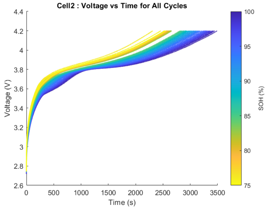
Figure A.1 Voltage profiles Cell 2 of Oxford are used to charge all the cycles.
