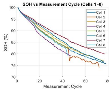
Fig. 3: SOH Degradation Curves of all 8 cells
