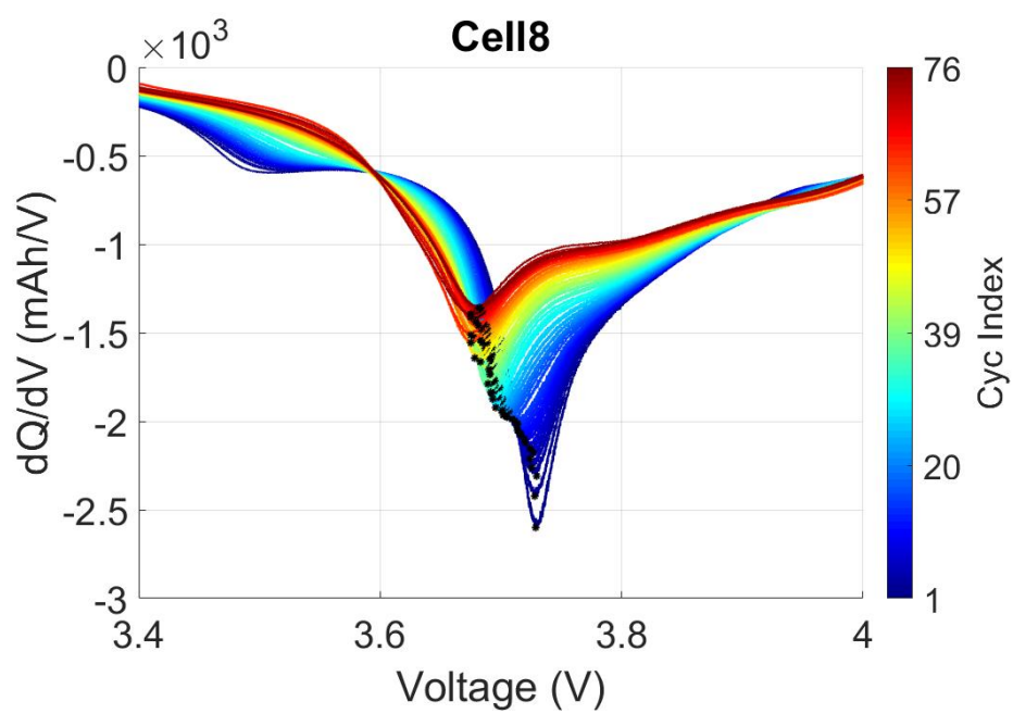
Figure C.7 ICA curves for Oxford Cell 8.
