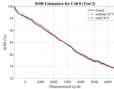
Fig. 8. SOH estimation of Cell 8 (Test 3).
