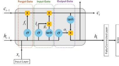
Fig.7: The LSTM Network Architecture
