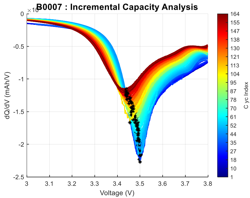
Figure D.2 ICA curves for NASA B0007.
