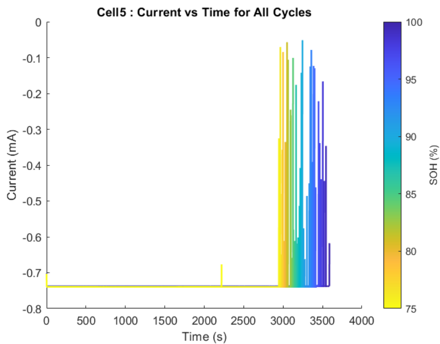
Figure A.25 Current profiles Cell 5 of Oxford are used to charge all the cycles.
