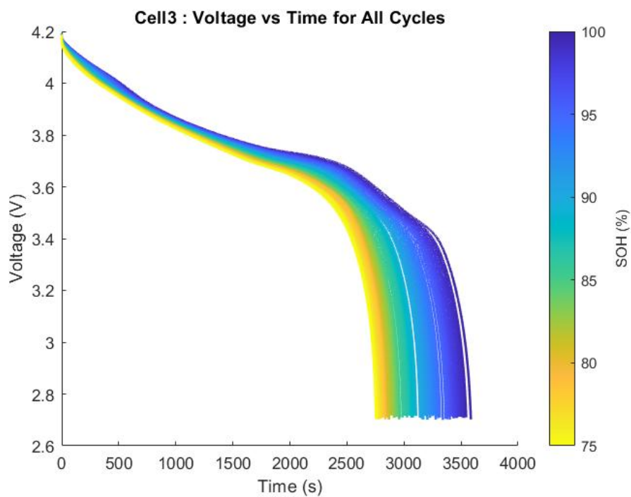
Figure A.9 Voltage profiles Cell 3 of Oxford are used to discharge all the cycles.
