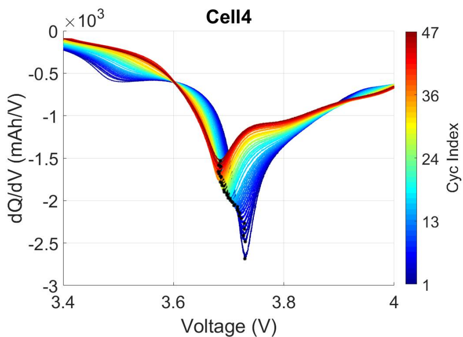
Figure C.3 ICA curves for Oxford Cell 4.
