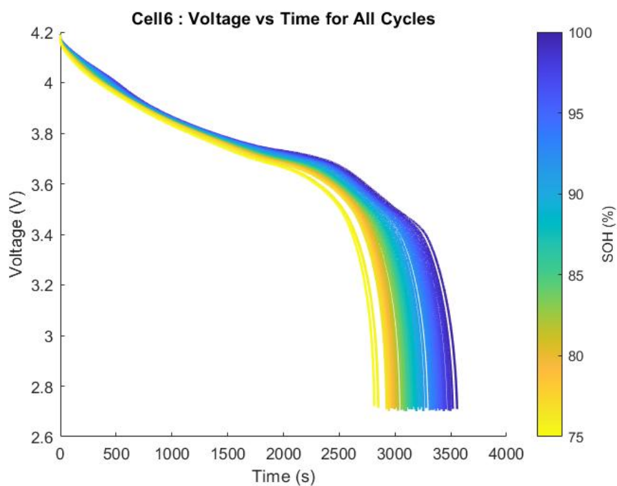
Figure A.12 Voltage profiles Cell 6 of Oxford are used to discharge all the cycles.
