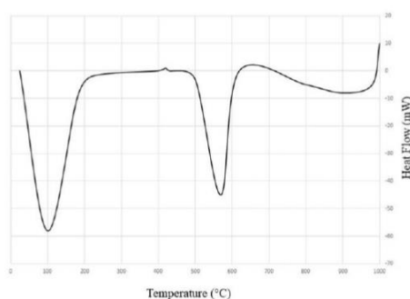
Figure 1. DTA curve of Narathiwat white clay.
