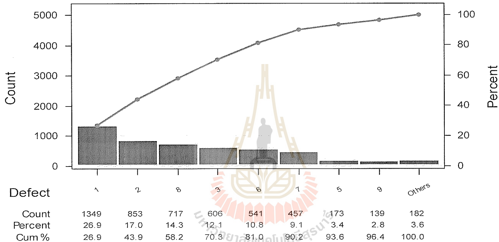
Parato Chart of % Brik Rework on 14 November to 14 December 2003
