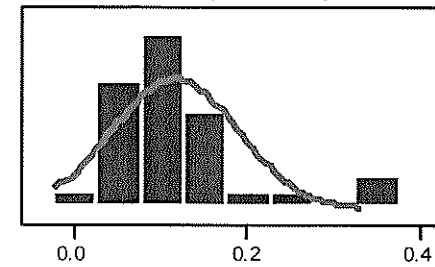
Normal Prob Plot
