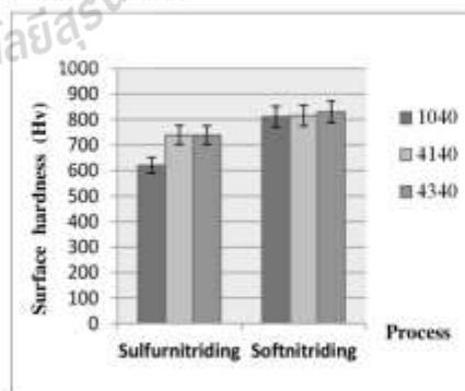
Fig. 4 Surface hardness of specimens
