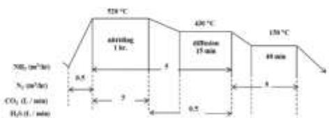
Fig. 2 Treatment conditions of sulfur-nitriding method
