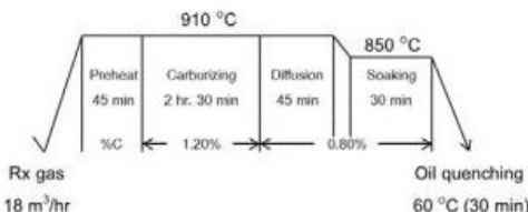
Fig. 2 Treatment conditions of carburizing method
