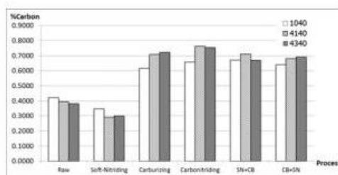
Fig. 4 Carbon content on surfaces of specimens
