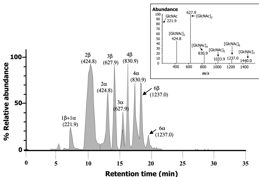
Fig. 7. A HPLC-MS chromatogram of hydrolytic products of chitinase A expressed in E. coli . Chitinase A (75 ng) was added to 100 \mu g/ml colloidal chitin and incubated at 20 ^{\circ} C for 5 min. After centrifugation, a 10-ml supernatant was immediately subjected to a hypercarb HPLC and eluted at 250 \mu l/min with a linear gradient from 5 to 40% acetonitrile into a LCQ ESI-MS. The relative abundance of the product peaks is plotted as a function of the elution time. Numbers indicate the amount of GlcNAc units in an oligomer, \alpha , and \beta indicate their isoforms. The inset represents the MS signal recorded in the SIM mode set for m/z 222, 425, 628, 831, 1034, and 1237.
