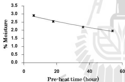
Fig. 5 Remaining moisture content of specimen no. 2.
