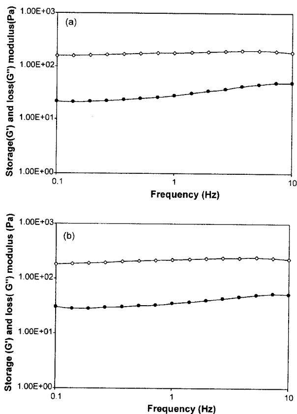
Fig. 6. Frequency dependence of storage ( G' , \diamond ) and loss ( G'' , \blacklozenge ) modulus of 1% (w/v) of Krueo Ma Noy pectin. (a) Crude extract, (b) dialyzed extract.
