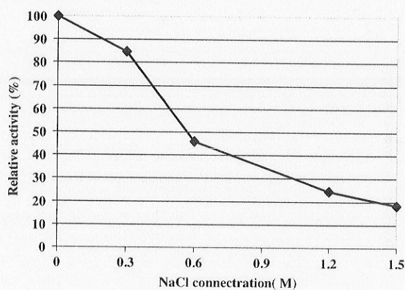
Fig. 10. Effect of NaCl on tilapia TGase activity.
