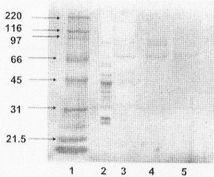
Fig. 4. SDS-PAGE of samples obtained from each purification step: lane 1, standard MW; lane 2, crude tilapia TGase; lane 3, DEAE-Sephacel; lane 4, Sephacryl S-200 HR; lane 5, HiTrap Heparin (purified TGase).
