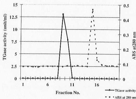
Fig. 2. Chromatogram of Tropical tilapia TGase on Sephacryl S-200 HR column.
