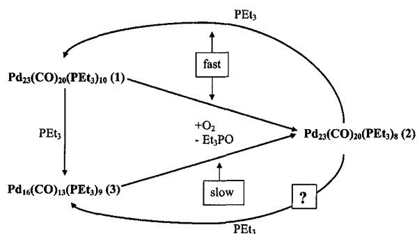
Fig. 4 Diagram summarizing observed interconversions among 1 , 2 , and 3 .
