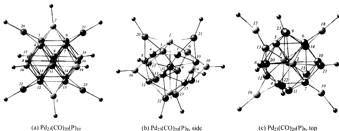
Fig. 1 Palladium-phosphorus frameworks of (a) \text{Pd}_{23}(\text{CO})_{20}(\text{PET}_3)_{10} ( 1 ) and of (b), (c) \text{Pd}_{23}(\text{CO})_{20}(\text{PET}_3)_8 ( 2 ) that stoichiometrically differ only by two additional \text{PET}_3 ligands attached to Pd(2) and Pd(3) in 1 . Atom-numbering establishes the structural relationship of the D_{2h} \text{Pd}_{23} core in 1 with the D_{2d} \text{Pd}_{23} core in 2 . Atom-coloring is based upon the centered hexacapped cuboctahedral geometry of \text{Pd}_{23}(\text{CO})_{20}(\text{PET}_3)_{10} ( 1 ). View (a) shows that the \text{Pd}_{23}(\text{P})_{10} fragment in 1 possesses a centered \text{Pd}_{13} cuboctahedral kernel consisting of an interior Pd(1) atom (red) coordinated to 12 ccp Pd( n ) atoms (blue). This \text{Pd}_{13} kernel of O_h symmetry is capped on each of its six square faces by Pd( n ) atoms ( n = 2, 3, 16-19 ; gold); the four remaining exopolyhedral edge-capping (wingtip) Pd( n ) atoms ( n = 20-23 ; green) located on a cuboctahedral mirror plane lower the symmetry from O_h to D_{2h} . Ten phosphorus atoms (violet) are attached to the six tetracapping and four wingtip Pd atoms. The nearly perpendicular views (b) and (c) show that the \text{Pd}_{23}(\text{P})_8 fragment in 2 may be described as a highly distorted centered hexacapped cubic \text{Pd}_{15} arrangement of 14 atoms (2 gold; 12 blue) connected to the centered Pd(1) atom (red); for clarity, connectivities are drawn between the interior Pd(1) atom (red) and two tetracapping axial Pd(2), Pd(3) atoms (gold) and four tetracapping horizontal Pd( n ) atoms ( n = 8-11 ; blue) but not between Pd(1) and eight geometrically deformed cubic corner Pd( n ) atoms ( n = 4-7, 12-15 ; blue). In turn, this \text{Pd}_{15} kernel is linked to four two-connected (wingtip) capping Pd( n ) atoms ( n = 16-19 ; gold) and four three-connected capping Pd( n ) atoms ( n = 20-23 ; green). The overall \text{Pd}_{23}(\text{P})_8 geometry ideally conforms to tetragonal D_{2d} symmetry with the improper S_4 axis passing through the centered Pd(1) (red) and Pd(2), Pd(3) (gold). View (c) approximately down the S_4 axis reveals that one of the two perpendicular \sigma_d mirror planes (that bisect the perpendicular pair of horizontal twofold axes) passes through Pd( n ) with n = 1, 2, 3, 9, 11, 22, 23 and the other \sigma_d through Pd( n ) with n = 1, 2, 3, 8, 10, 20 and 21. This idealized metal-core conformity of 2 to D_{2d} symmetry is based upon the inherent assumption that the four Pd( n ) atoms ( n = 20-23 ) related by the S_4 axis can be viewed as tetracapping instead of tricapping connected atoms (see text).
