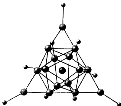
Fig. 3 Palladium-phosphorus framework of the known \text{Pd}_{16}(\text{CO})_{13}(\text{PEt}_3)_9 cluster 4 showing the central atom (red) encapsulated by an icosahedral \text{Pd}_{12} cage (brown) with three additional exopolyhedral edge-bridged (wingtip) Pd atoms (green). Alkyl substituents on phosphorus atoms (violet) and eight doubly and five triply bridging carbonyl ligands are omitted.
