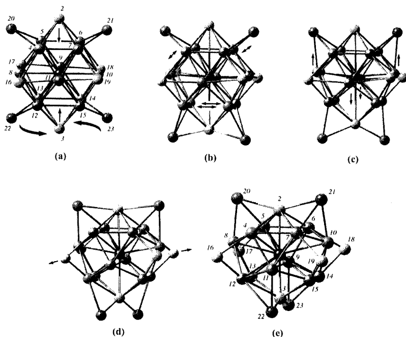
Fig. 2 Four-stage structural diagram showing the geometrical relationship between the structurally dissimilar Pd 23 cores of Pd 23 (CO) 20 (PEt 3 ) 10 ( 1 ) and Pd 23 (CO) 20 (PEt 3 ) 8 ( 2 ). Although possible intermolecular , transformations have not been experimentally excluded, this hypothetical, geometrical transformation illustrates the possible intramolecular pathway that preserves maximum connectivities upon removal of the two phosphine ligands via reaction with O 2 (air). Stages (a) and (e) correspond to the metal-core geometries of 1 and 2 , respectively, with the same numbering of corresponding atoms as presented in Fig. 1 for both structures. Arrows point to the types of structural distortions. Bond-cleavage of two PEt 3 ligands from trans , tetracapping Pd(2), Pd(3) atoms (gold) of the D 2h Pd 23 core-geometry in 1 and resulting formation of the D 2d Pd 23 core-geometry in 2 are proposed to proceed from stage (a) to stage (e) by intermediate snapshot stages (b)–(d). Although the stages in this least-nuclear-motion scheme are shown consecutively, the occurrence of an intramolecular transformation would no doubt involve an essentially simultaneous combination ( i.e. , concerted process) of all stages. Each stage-transformation involves the formation and scission of particular atom-pair connectivities. (1) (a) to (b) transformation: 1–2; 1–3; 3–22; 3–23 connectivities formed. 4 ··· 5; 6 ··· 7; 13 ··· 14; 12 ··· 15 connectivities broken. (2) (b) to (c) transformation: 8–20; 10–21 connectivities formed. 22 ··· 13; 23 ··· 15 connectivities broken upon commencement of counterclockwise 90° rotation of connected Pd(22)–Pd(3)–Pd(23) fragment about the S 4 Pd(3)–Pd(1)–Pd(2) axis. (3) (c) to (d) transformation: continuation of 90° rotation of connected Pd(22)–Pd(3)–Pd(23) fragment about the S 4 axis. 2–20; 2–21 connectivities formed. 4 ··· 20; 6 ··· 21; 8 ··· 16,17; 9 ··· 17,18; 10 ··· 18,19; 11 ··· 16,19 connectivities broken. (4) (d) to (e) transformation: completion of 90° rotation of Pd(22)–Pd(3)–Pd(23) fragment about S 4 axis. 22–11; 23–9 connectivities formed. The total number of Pd–Pd bonding connectivities has significantly decreased in the formation of 2 , from 68 in 1 to 62 in 2 . Noteworthy is that mean Pd–Pd bonding connectivities range from 2.68 to 2.97 Å; mean Pd–Pd distances >3.22 Å are designated as non-bonding connectivities. This arbitrary distinction gives rise to the formulation of four wingtip (edge-capping) Pd(μ 2 -CO) 2 (PR 3 ) fragments ( n = 20–23) in 2 .
