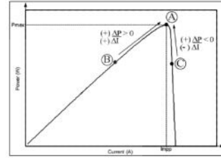
Fig. 3. P-I curve of PV panel for current based
