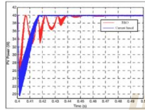
Fig. 10. Power transient at irradiance 1000 W/m²
