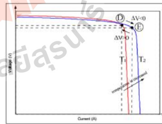
Fig. 5. V-I curve for temperature variation
