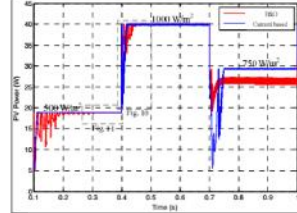
Fig. 9. Simulation result of compare P&amp;O and current based
